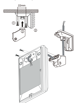
Ceiling mounting
