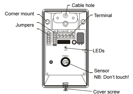
Wall mounting
